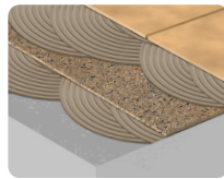
Double-Bond Compatible
